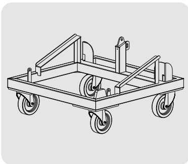
CA-4LAIA28 Transport dolly for up to 4 LAIA-28.
